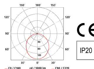
VINDO R 22 LED 10 W 108 lm/W
